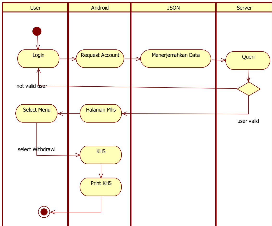
Gambar 2. Activity Diagram Fitur KHS
