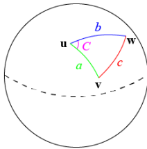
Gambar Ilustrasi Spherical law of cosines
