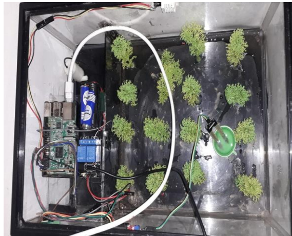
Gambar 2. Desain hardware
