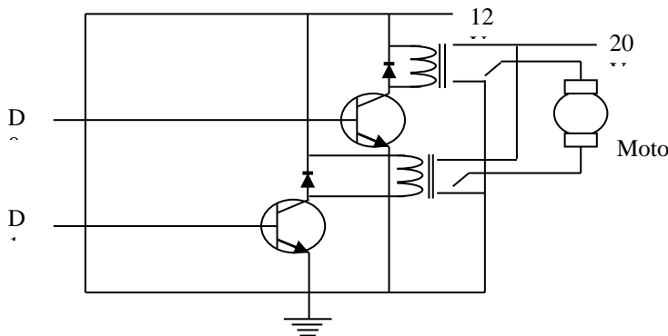
Gambar Rangkaian Driver
