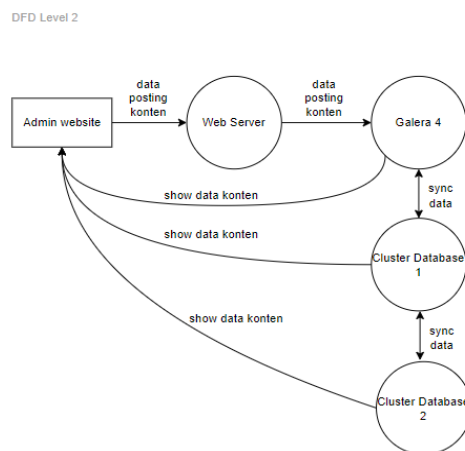
Gambar 6. DFD Level 2
