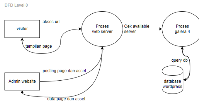
Gambar 4. DFD Level 0
