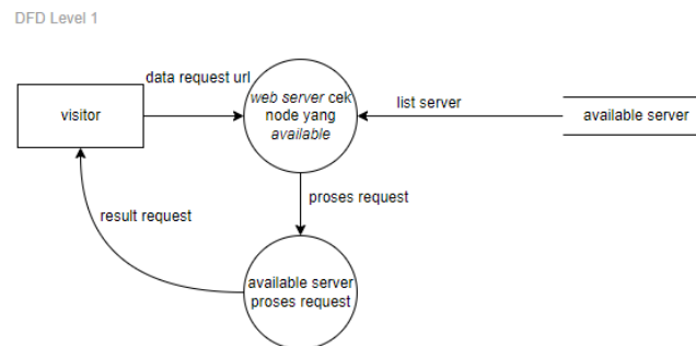
Gambar 5. DFD Level 1
