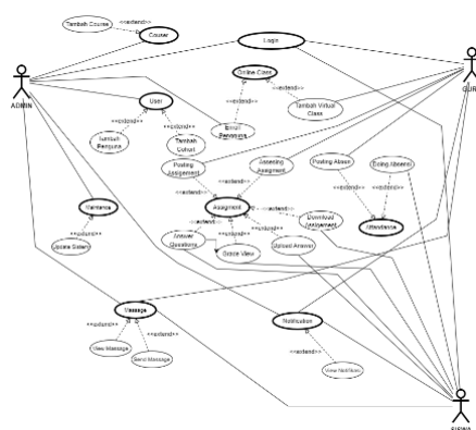
Gambar 2. Diagram Use Case LMS
